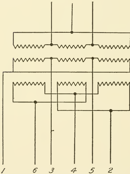
Fig. 35.—Six-Phase \Delta Circuit for Transformer with Two Secondaries
